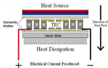
Figure 1. Thermoelectric power generation structure [4]
