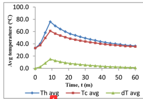
Figure 4. History of average hot side temperature ( T_h avg), average cold side temperature ( T_c avg) and average temperature difference ( dT avg) at 1 m chimney height.
